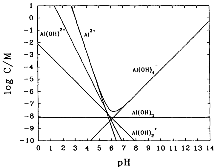
Fig. 1. Solution state of \text{Al}^{\text{III}} in the absence of strongly coordinating agents (see text), as predicted from thermodynamic data (23). In the formulas, metal-coordinated water molecules are omitted.
